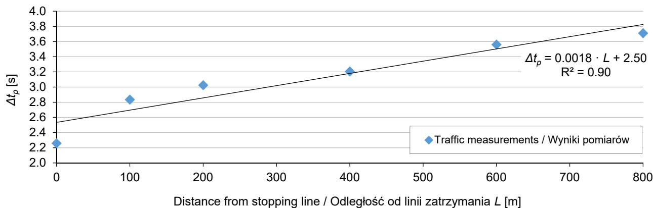
Fig. 6. Average headway between vehicles moving in the queue
