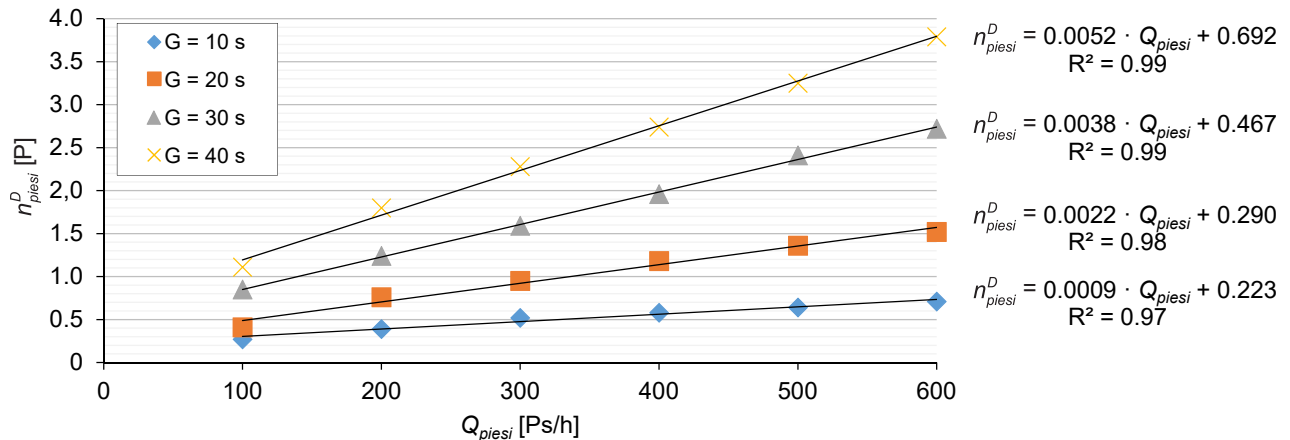
Fig. 4. The influence of pedestrian traffic volume Q_{piesi} and duration of green signal G^B on the number of vehicles from entry D joining the queue
