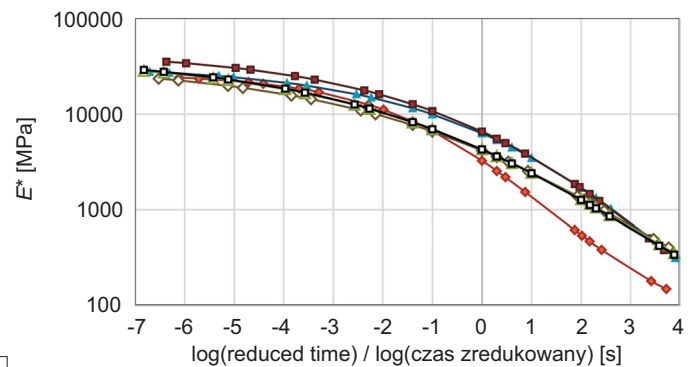
Fig. 4. Example of master curves for asphalt mixtures designed acc. to Polish standards (Level 1) in comparison with default master curves (Level 3), mixtures tested acc. to procedure [13]
