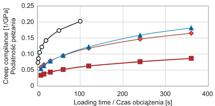
Fig. 3. Example of creep compliance at -10^{\circ}\text{C} for asphalt mixtures designed acc. to Polish standards (Level 1) in comparison with default creep compliance curve (Level 3), mixtures tested acc. to procedure [12]
