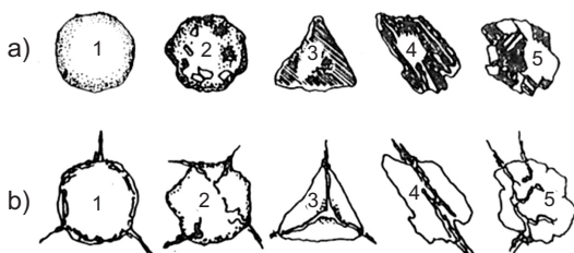
Fig. 1. Grains of aggregate with different mineral composition and morphology: a) initial condition, b) with ASR - induced characteristic micro-cracks [19]
