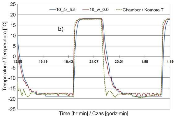
Fig. 8. Change of ambient temperature and temperature inside the specimens of 100 mm side (a) and 150 mm side (b) placed in the temperature chamber during standard freeze-thaw durability tests according to PN-B-06250
