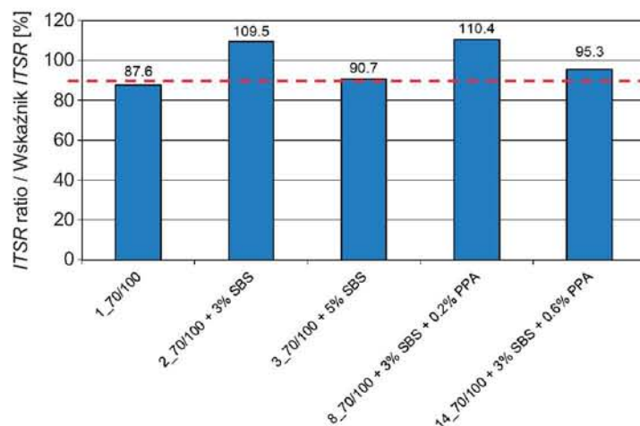
Fig. 10. Test results of ITSR indicator of SMA 8 mixture as a function of used binder
