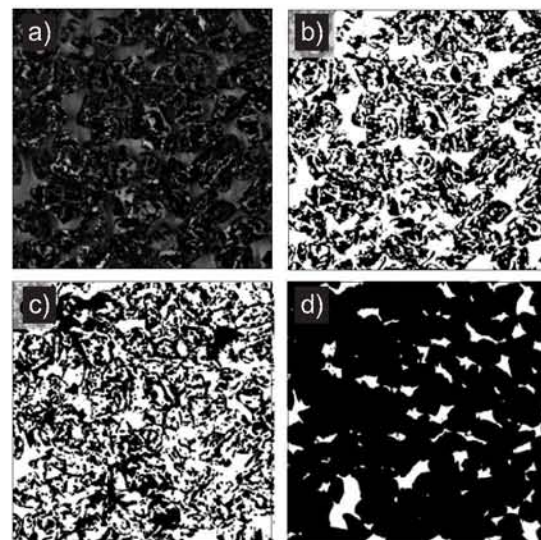
Fig. 3. a) a digital image of the sample after the stripping test in 8-bit grayscale, b) phase 1: the binary image on the binder (black), c) phase 2: the binary image on stripped aggregate (black), d) phase 3: the binary image on the entire sample, without the background (black) [3]
