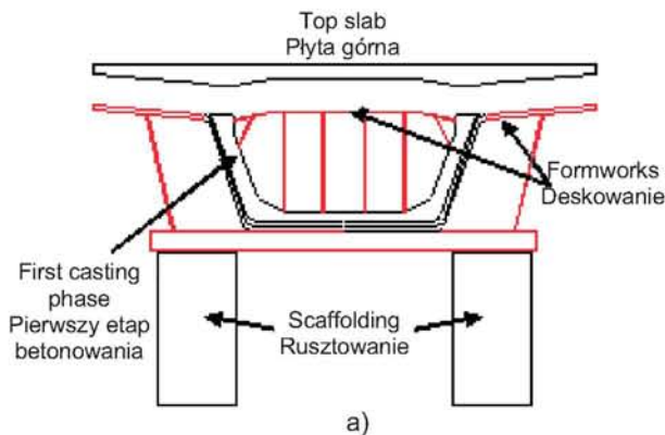
Fig. 1. Scheme of the top slab weight distribution between the U-section and scaffolding
