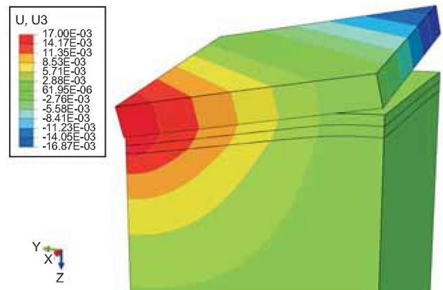
Fig. 9. Contours of rigid pavement vertical displacements - II variant (contact modelling); deformation scale factor 50
