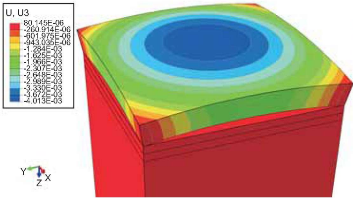
Fig. 10. Contours of vertical displacements for rigid pavement under temperature gradient - III variant (contact modelling); deformation scale factor 100
