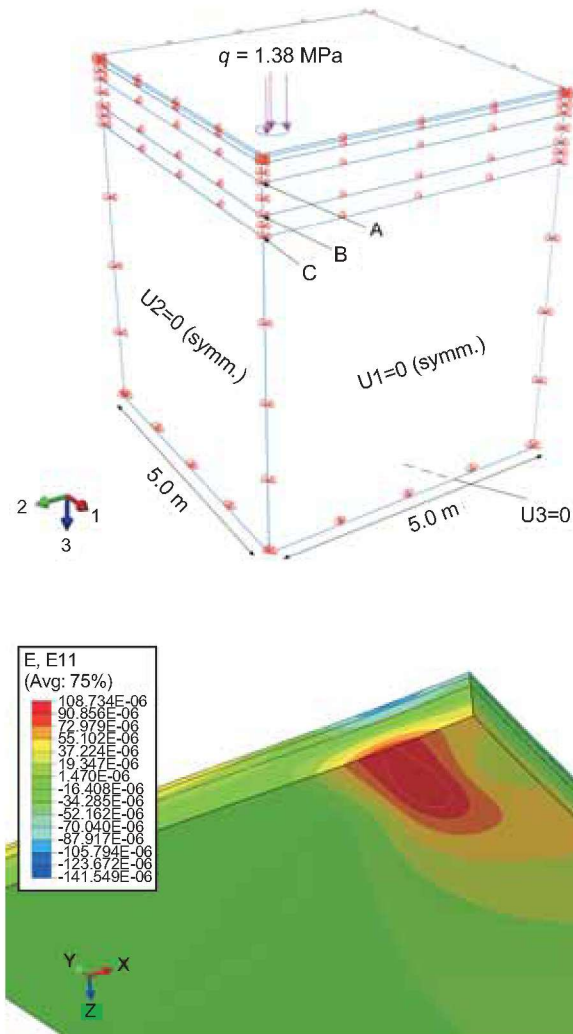
Fig. 16. Contours of horizontal strain component \varepsilon_{xx} at the bottom of asphalt concrete base - model with 30 cm layer of improved subgrade
