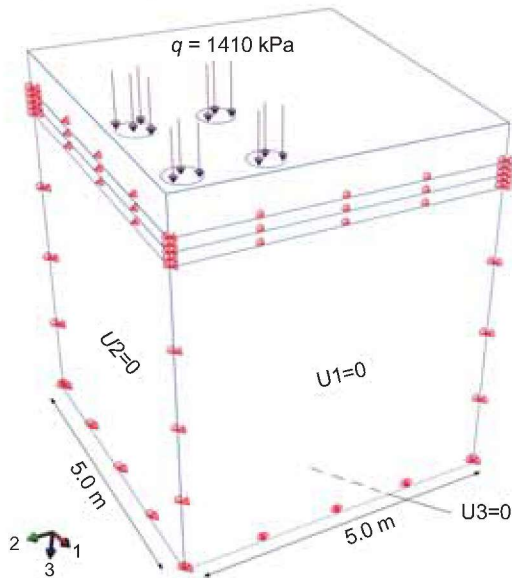
Fig. 5. Geometry of rigid pavement model with boundary conditions and loading scheme
