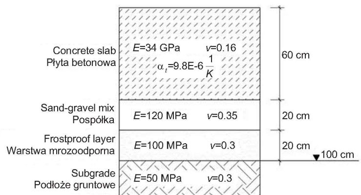
Fig. 2. Layered structure of rigid aircraft pavement
